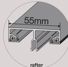
rafter 2 x Rafter Outer
